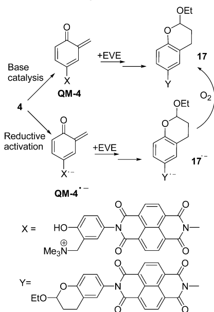
SCHEME 5. Reactivity of QM-4 and QM-4 •− as Heterodiene in a [4 + 2] Cycloaddition
