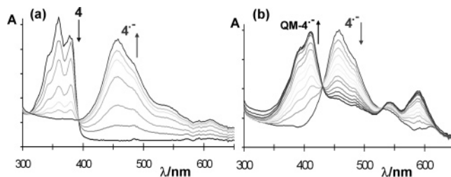
FIGURE 1. Generation from 0 to 20 min (a) and reactivity from the following 2 h (b) of 4 •− monitored by UV–visible spectroscopy.
