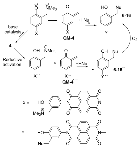
SCHEME 4. Base Catalytic and Reductive Activation of 4 as Bisalkylating Agent through the Generation of QM-4 and QM-4 •-
