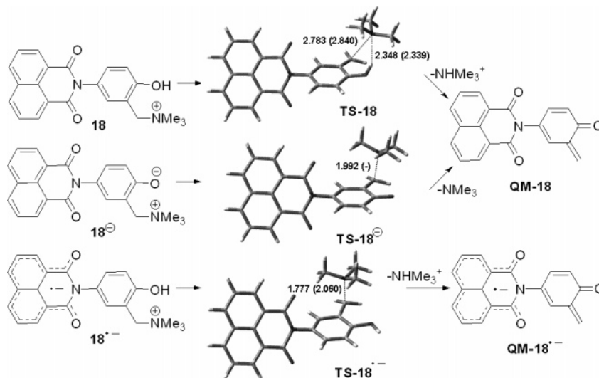
SCHEME 6. Generation of QM-18 and QM-18 •- through the TSs TS-18, TS-18 - , and TS-18 •- (Bond Lengths are in Angstroms; Data in Parentheses are for Full R(U)B3LYP/6-31+G(d,p) Optimization in Aqueous Solution)
